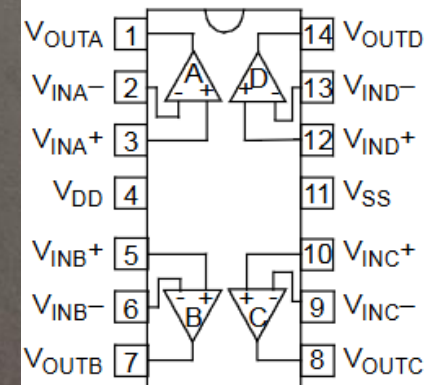
MCP6004 PDIP, SOIC, TSSOP
